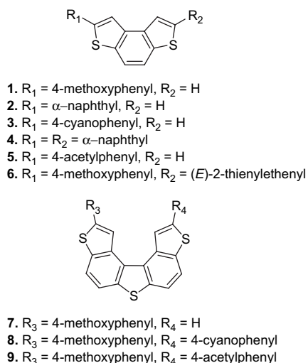
Chart 1. Molecular structures of BDT and T5H derivatives 1–9 .
