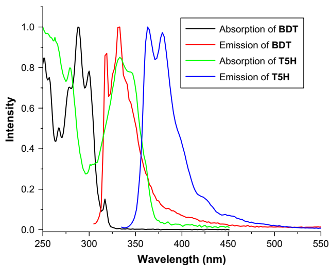
Figure 5. Normalized absorption and emission spectra of BDT and T5H in \text{CH}_2\text{Cl}_2 .
