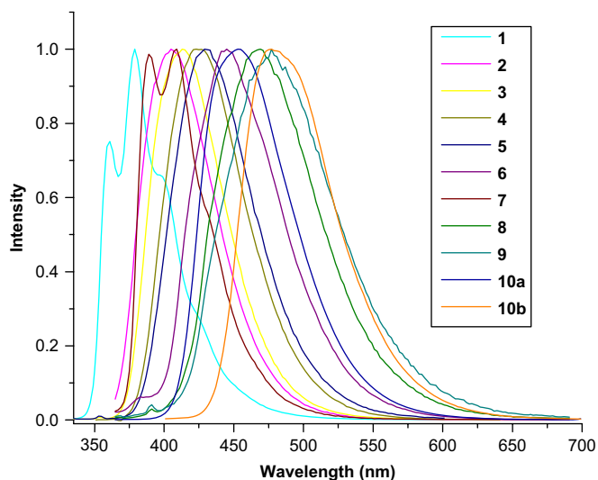
Figure 6. Normalized fluorescence spectra of compounds 1–10b in \text{CH}_2\text{Cl}_2 solution at room temperature.
