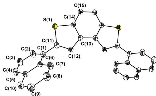
Figure 2. X-ray crystal structure of 4 .
