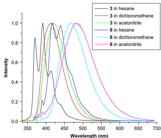
Figure 7. Normalized fluorescence spectra of compounds 3 and 8 in different solvents.
