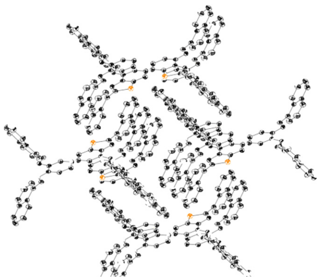
Figure 3. Packing pattern of 4 .
